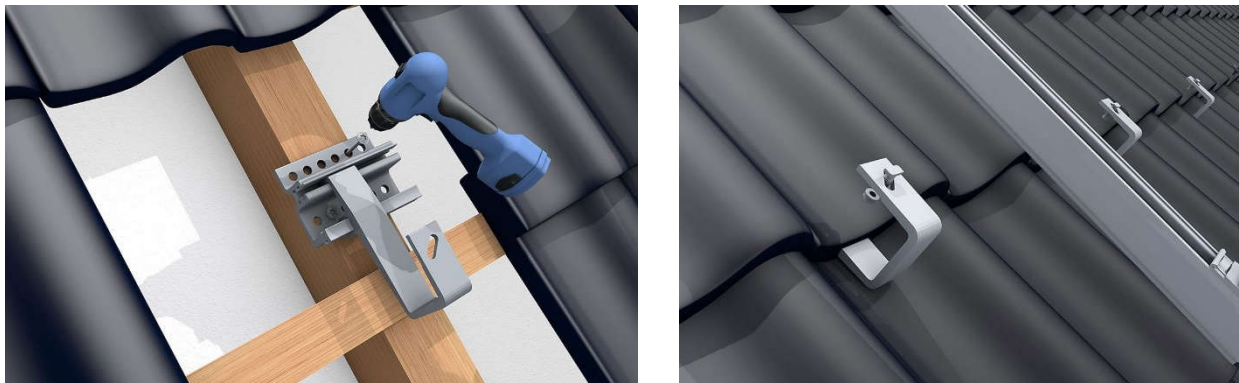
Figure 4-1 Sketch of the substructure installation on the roof (Source: https://www.tritec-energy.com/en/ )
