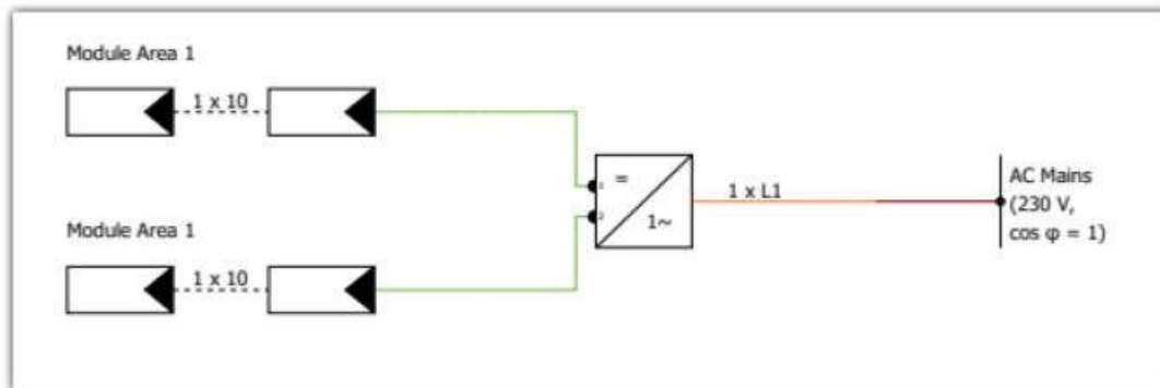
Figure 4-3 Single-pole circuit diagram of the PV module and the exchanger
