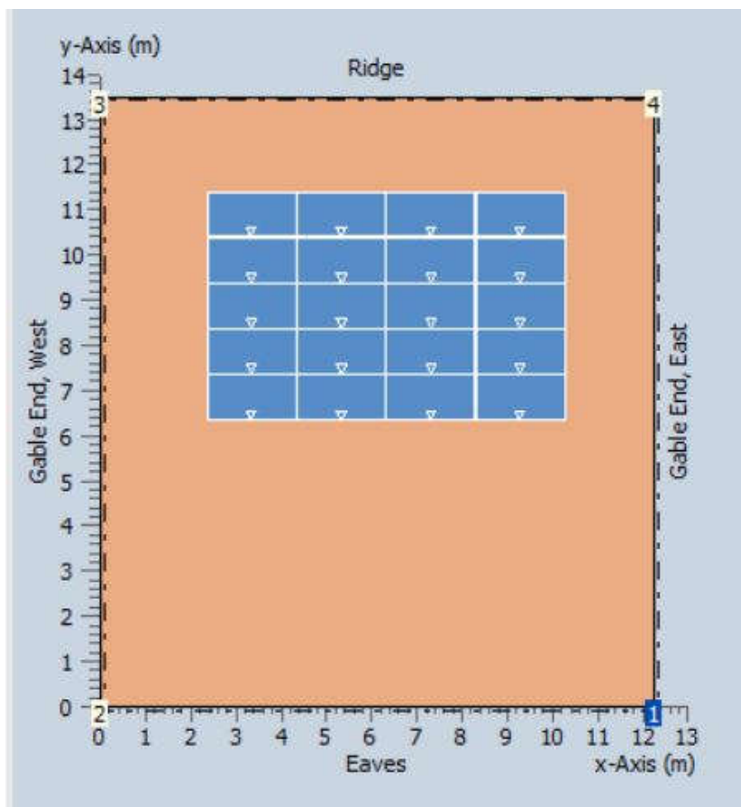
Figure 4-2 Elements layout on the roof of DV Osmjeh power plant
