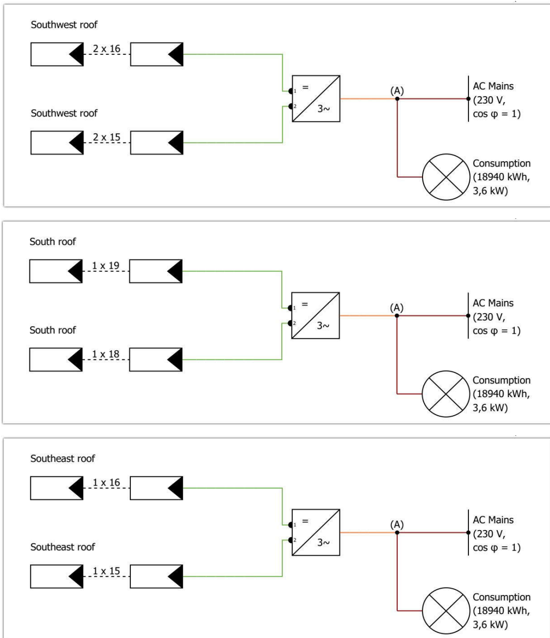
Figure 4-3 Single-pole circuit diagram of the PV modules and the exchanger1, exchanger2 and exchanger3
