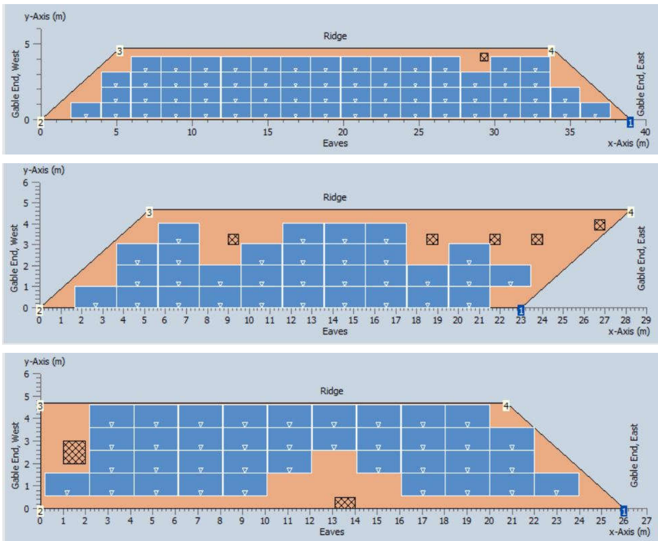
Figure 4-2 Elements layout on the roof of KS Bertoki power plant (southwest part of the roof, southeast part of the roof, south part of the roof)
