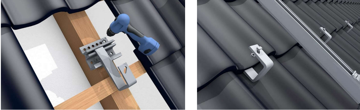
Figure 4-1 Sketch of the substructure installation on the roof (Source: https://www.tritec-energy.com/en/ )
