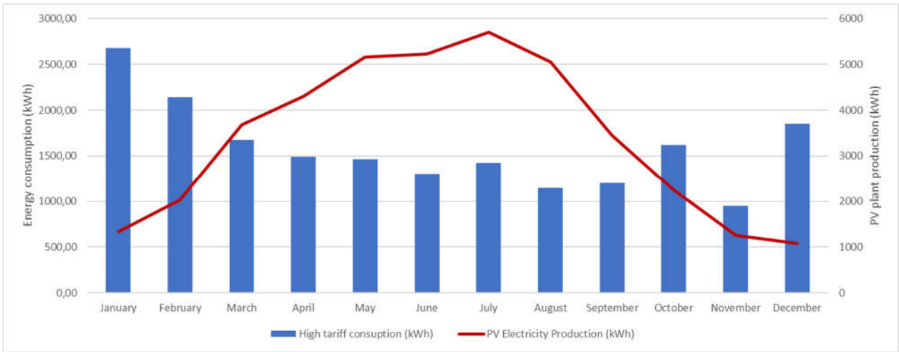
Figure 5-3 Monthly consumption in relation to PV production for KS Bertoki
